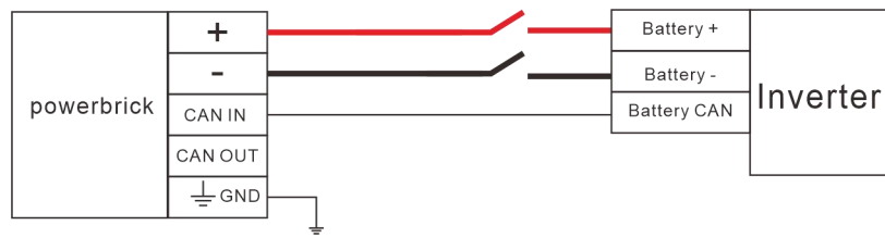
Figure 3-5 Wiring diagram
