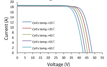
Current-Voltage (700W)
